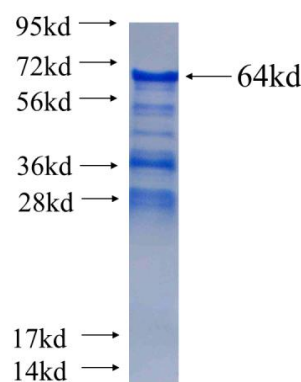
Recombinant human MLL5 SDS-PAGE
