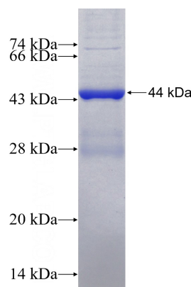
Recombinant Human NFKBIZ SDS-PAGE
