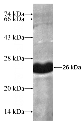
Recombinant Human RHBDL3 SDS-PAGE
