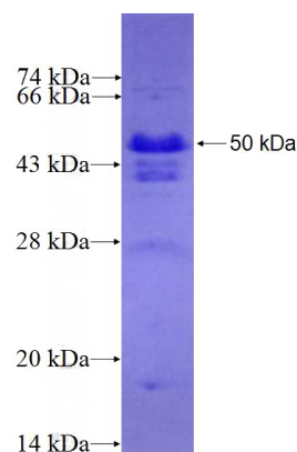
Recombinant Human AMOT SDS-PAGE
