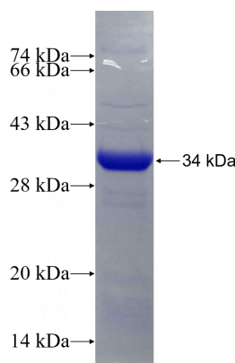
Recombinant Human RNASEH2A SDS-PAGE
