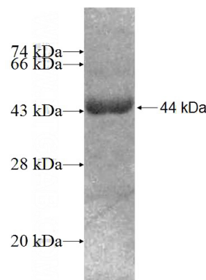
Recombinant Human UBA7 SDS-PAGE
