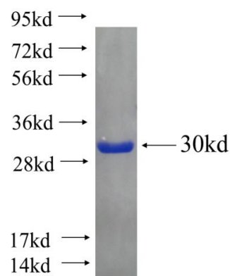
Recombinant human APOL6 SDS-PAGE
