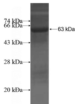
Recombinant Human WWP1 SDS-PAGE
