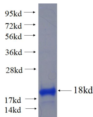
Recombinant human RPTN SDS-PAGE
