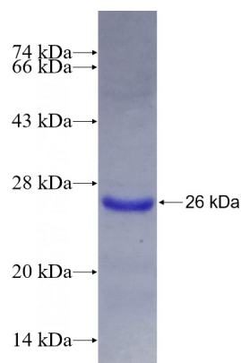
Recombinant Human SOCS2 SDS-PAGE
