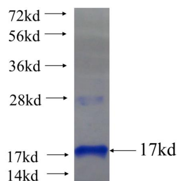
Recombinant human ORAI3 SDS-PAGE
