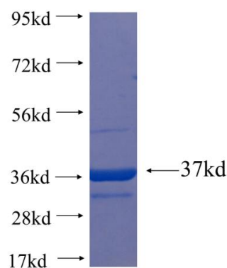
Recombinant Arabidopsis thaliana NF-YB2 SDS-PAGE
