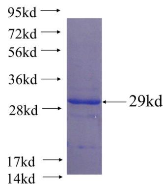
Recombinant human TMEM199(Full length) SDS-PAGE
