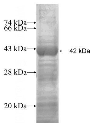
Recombinant Human PDE11A SDS-PAGE
