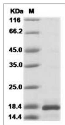
Pfdn1 protein SDS-PAGE
