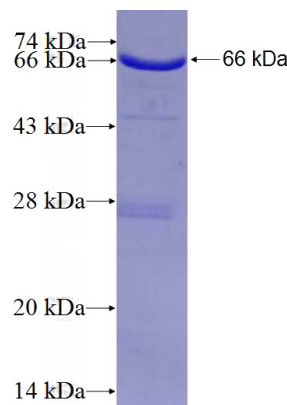
Recombinant Human GSPT1 SDS-PAGE
