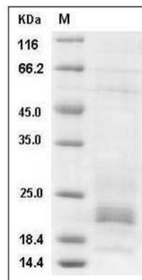
Mouse IFNG / Interferon Gamma Protein (His Tag) SDS-PAGE
