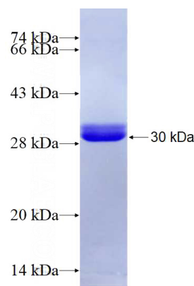
Recombinant Human DMXL2 SDS-PAGE
