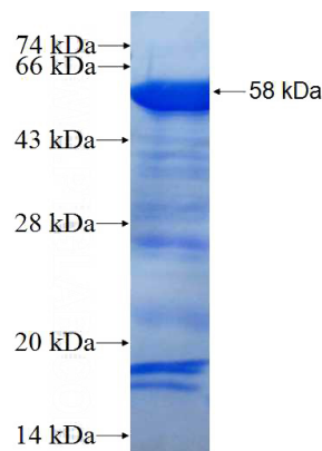
Recombinant Human IRF4 SDS-PAGE
