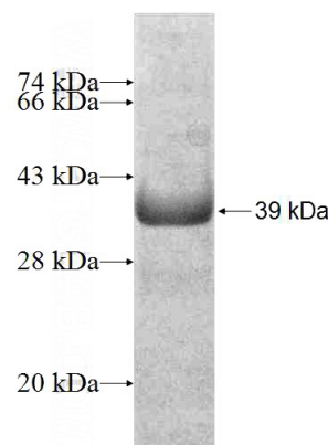
Recombinant Human CAPZA2 SDS-PAGE
