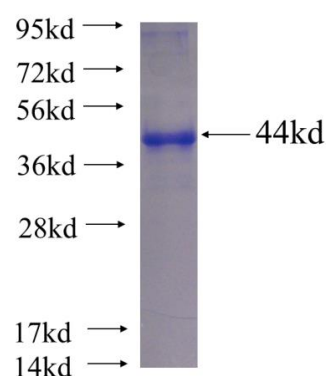
Recombinant human AXIN1 SDS-PAGE
