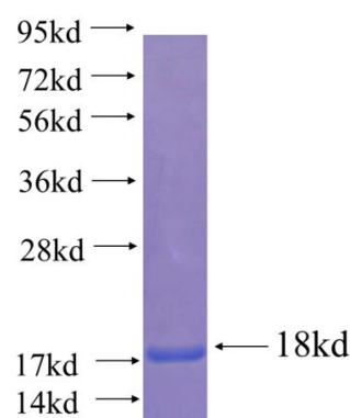
Recombinant human CCDC21 SDS-PAGE
