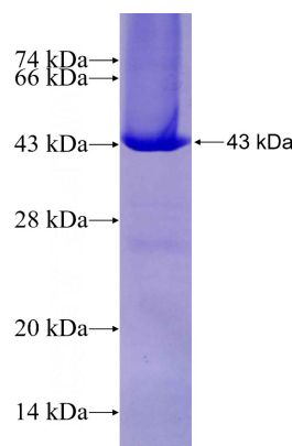
Recombinant Human Syntaxin 18 SDS-PAGE
