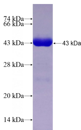
Recombinant Human SRGAP3 SDS-PAGE
