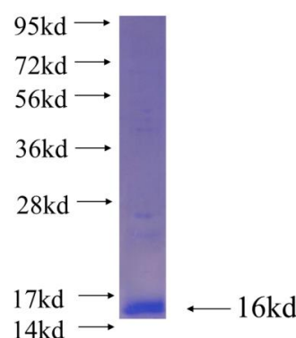
Recombinant human GALR2 SDS-PAGE
