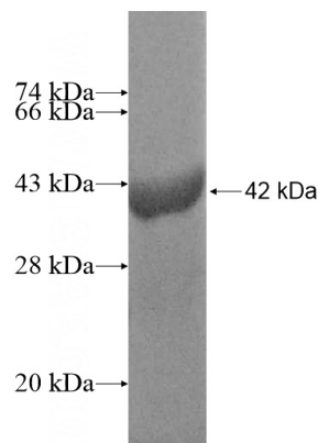
Recombinant Human LRRN1 SDS-PAGE
