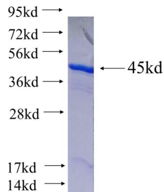
Recombinant human MAGEB18(Full length) SDS-PAGE
