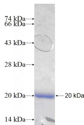
Recombinant Human TRMT2B SDS-PAGE
