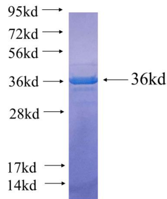
Recombinant human MAPK8IP2 SDS-PAGE
