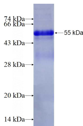
Recombinant Human C5, C5a SDS-PAGE
