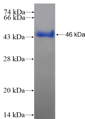
Recombinant Human ATP6V0D1 SDS-PAGE
