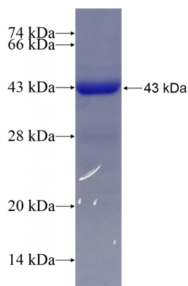
Recombinant Human CYP17A1 SDS-PAGE
