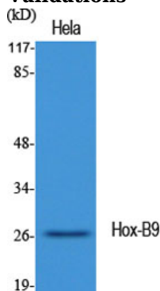
Fig1.; Western Blot analysis of various cells using Hox-B9 Polyclonal Antibody diluted at 1: 1000 cells nucleus extracted by Minute TM Cytoplasmic and Nuclear Fractionation kit (SC-003, Inventbiotech, MN, USA).
