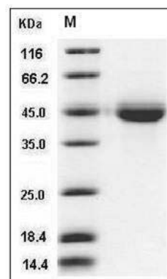
Human VSIG4 Protein (His Tag) SDS-PAGE
