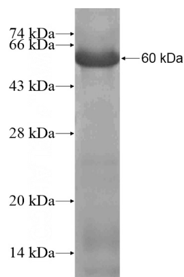
Recombinant Human ZNF335 SDS-PAGE
