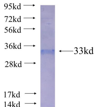
Recombinant human GNG3 SDS-PAGE
