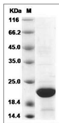
Human XTP3TPA / DCTPP1 Protein (His Tag) SDS-PAGE
