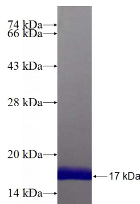
Recombinant Human CHCHD5 SDS-PAGE
