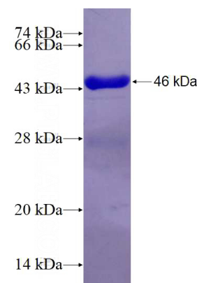
Recombinant Human KCNN1 SDS-PAGE
