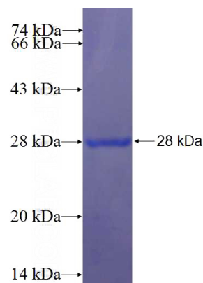
Recombinant Human BAIAP2L1 SDS-PAGE
