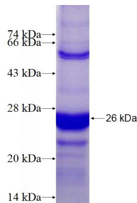
Recombinant Human ANKRD7 SDS-PAGE
