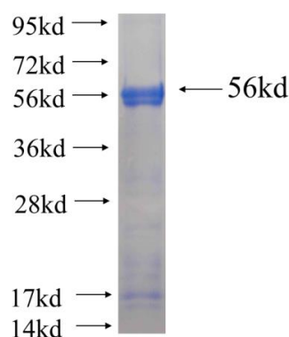
Recombinant Arabidopsis thaliana ATSUFS SDS-PAGE
