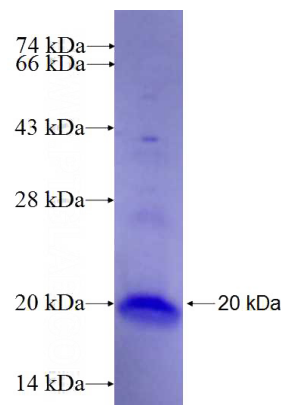
Recombinant Human THAP7 SDS-PAGE
