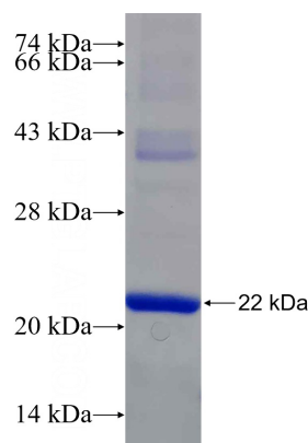
Recombinant Human SEC22A SDS-PAGE
