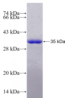
Recombinant Human PCM1 SDS-PAGE
