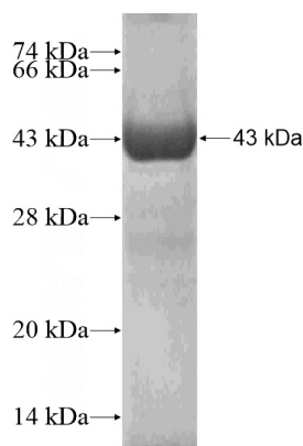
Recombinant Human CYP7B1 SDS-PAGE
