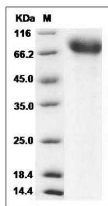
Mouse TrkA / NTRK1 Protein (His Tag) SDS-PAGE
