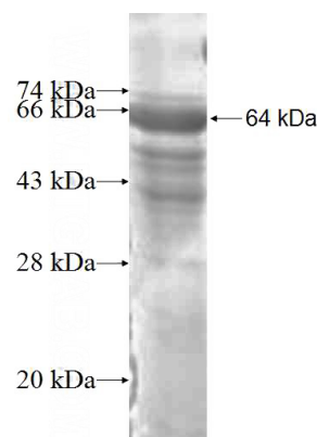
Recombinant Human UBOX5 SDS-PAGE
