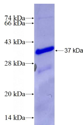
Recombinant Human TCF7L1 SDS-PAGE
