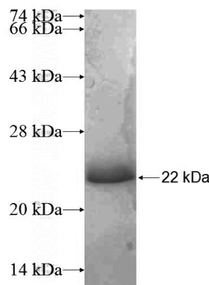
Recombinant Human SLC38A10 SDS-PAGE
